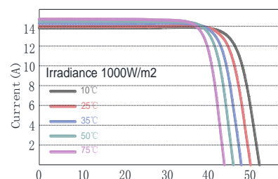
Voltage current curve at different temperatures
