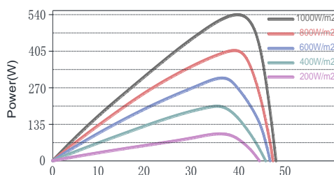
Power-Voltage Curver
