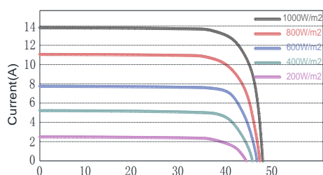
Current-Voltage Curver
