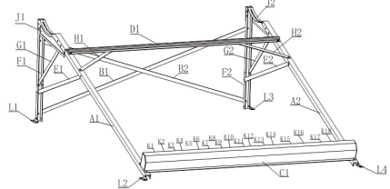
U Type Bracket
